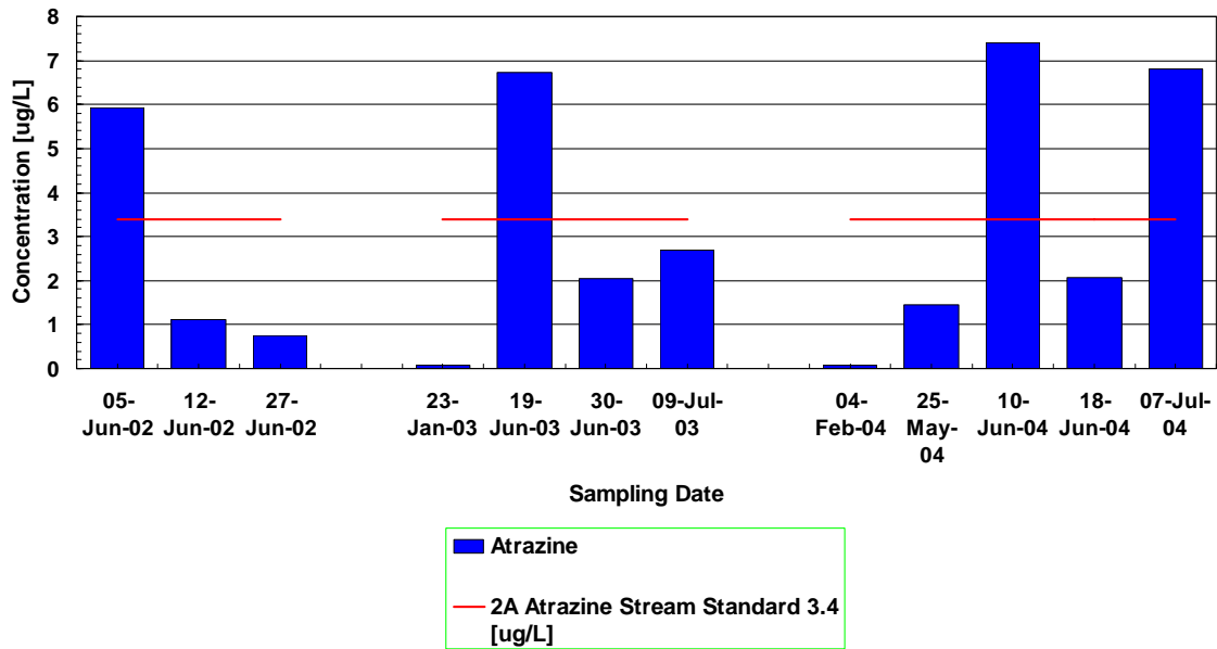
Figure 27. Atrazine concentrations in the South Branch of the Root River over time.
